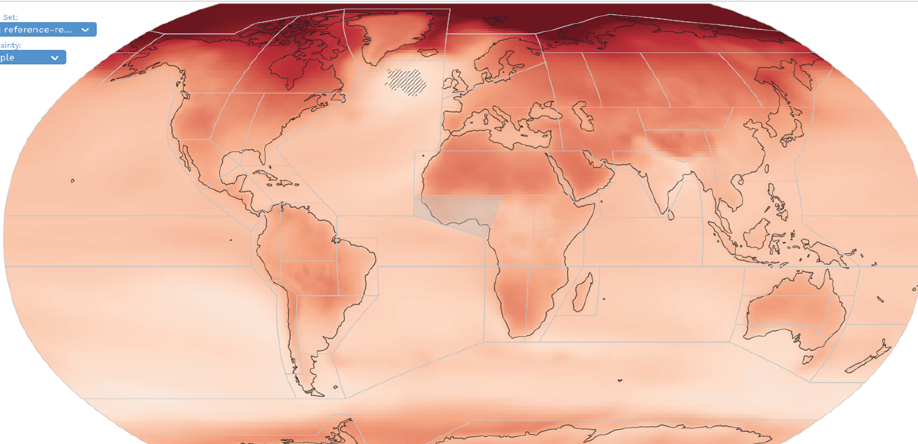
CMIP6 - Mean temperature (T) Change deg C - Warming 2°C SSP5 8.5 (rel. to 1850-1900) - Annual (34 models)
