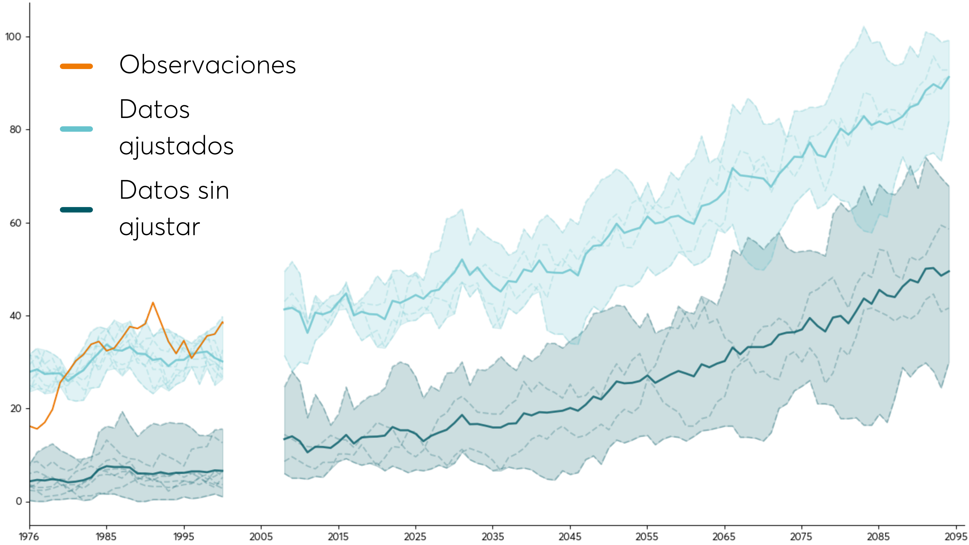
Number of days above 30 °C (RCP85 and historical scenarios) in Valderredible (Spain)
